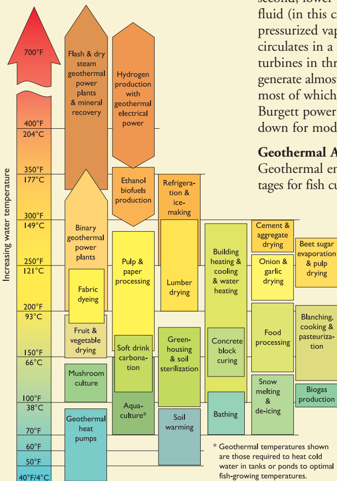
Temperature ranges of applications ideally suited to geothermal energy (modified from Geothermal Energy Uses , courtesy of the Geothermal Education Office, 2005).
